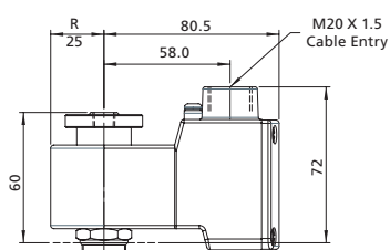
Solenoid Code P&T
