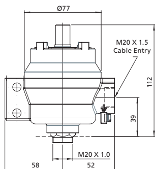
Solenoid Code K&7
